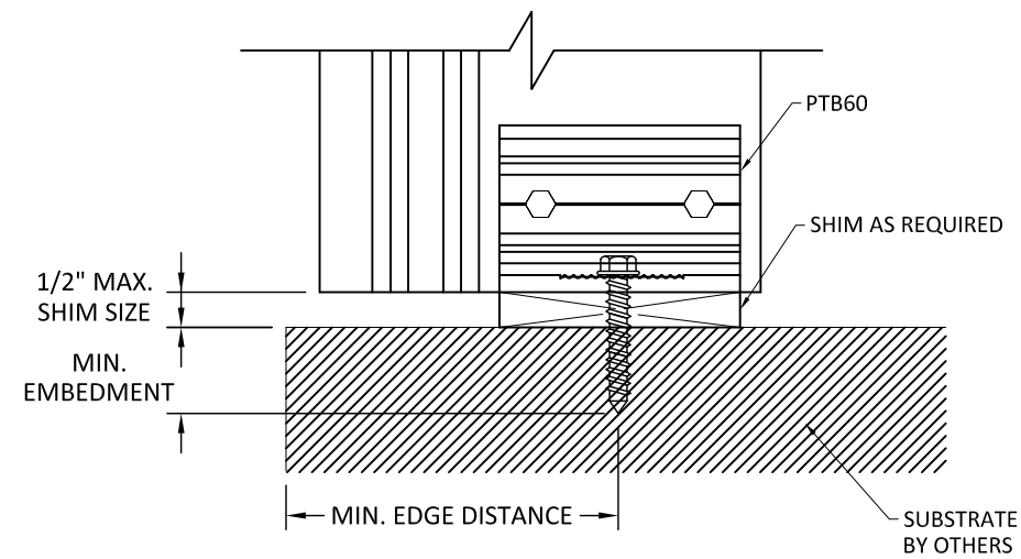
2 7.2 SIDE VIEW FRAME CLIP CONNECTION
