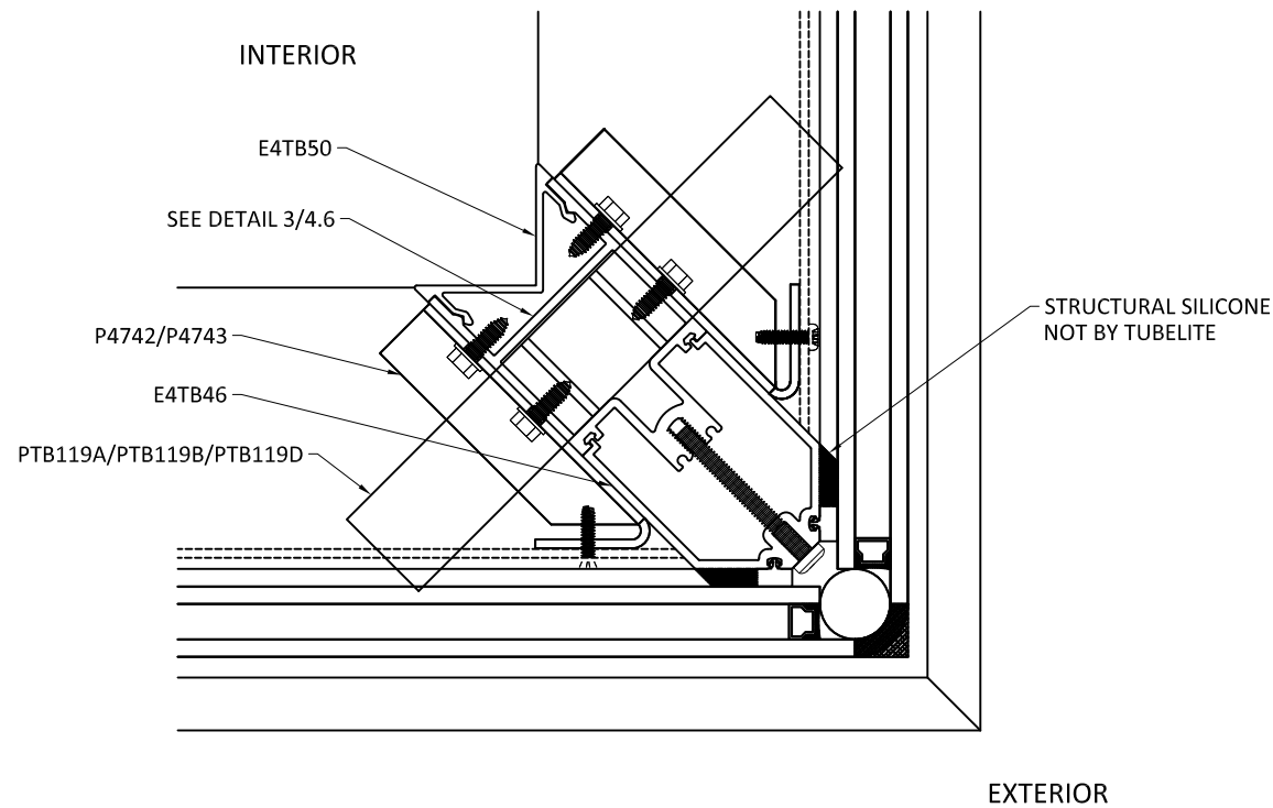
1 4.6 OUTSIDE CORNER STRUCTURAL SILICONE GLAZE
