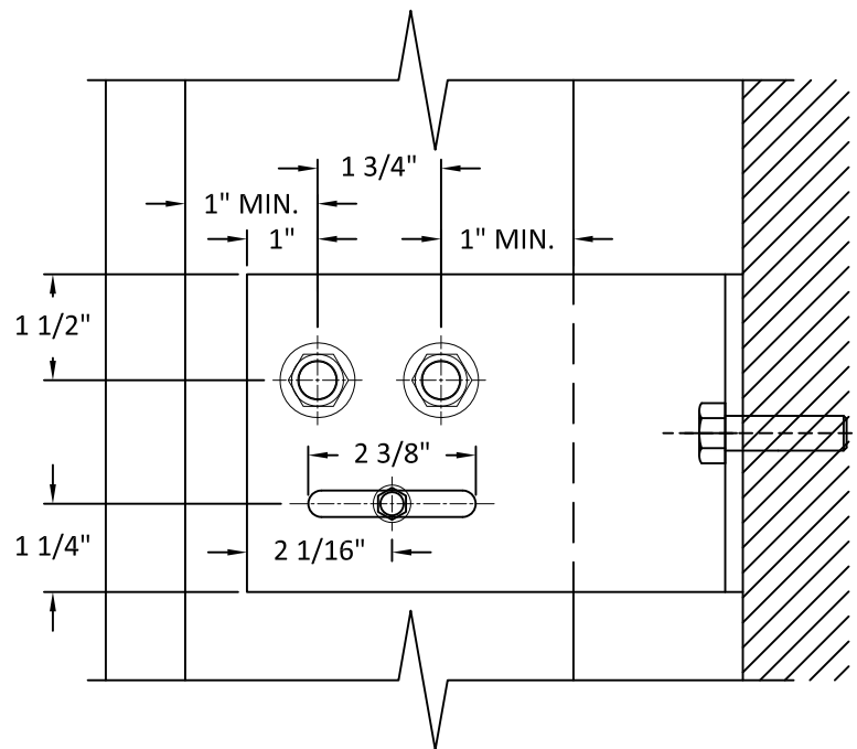
DEAD LOAD ANCHOR SIDE VIEW
