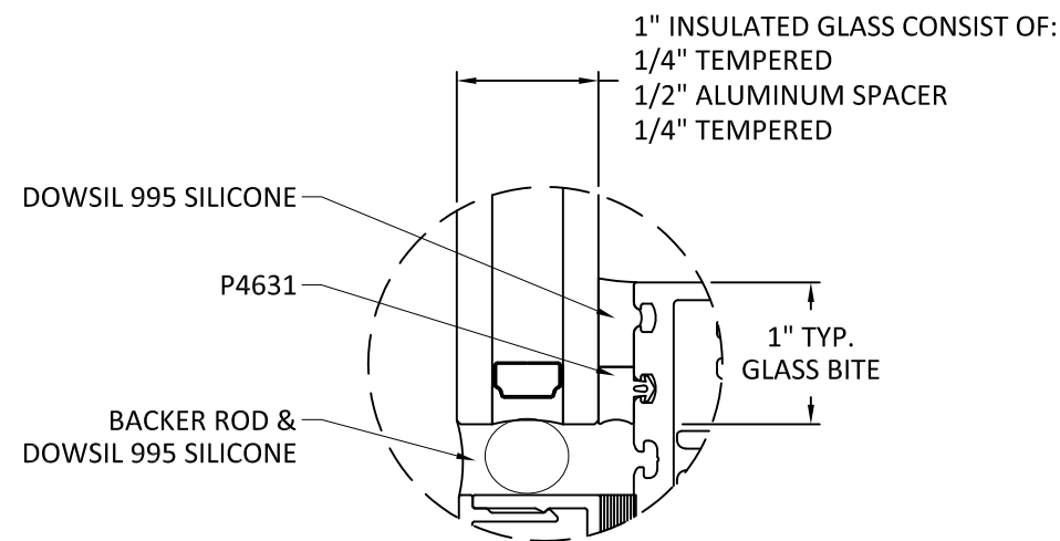
GLAZING DETAILS
