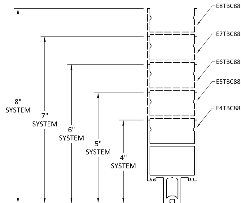
3 4.6 CORNER PROFILES
