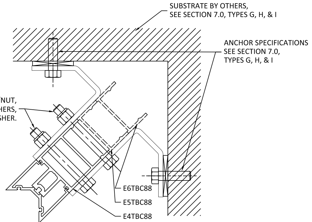
2 8.1 VERTICAL SECTION WIND/DEAD LOAD ANCHOR AT CORNER
