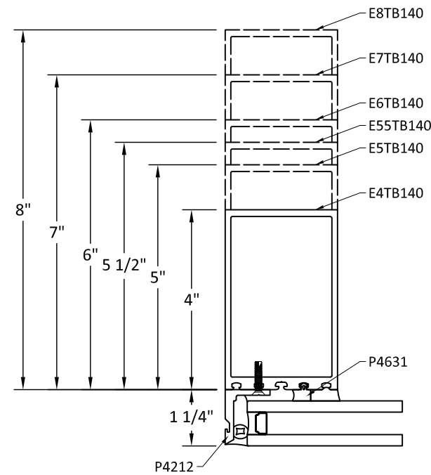
JAMB STRUCTURAL SILICONE GLAZE GLASS TO EDGE
