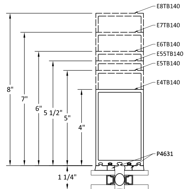
1 4.3 VERTICAL MULLION STRUCTURAL SILICONE GLAZE
