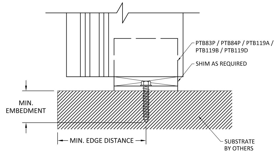
1 7.2 SIDE VIEW F/T ANCHOR CONNECTION
