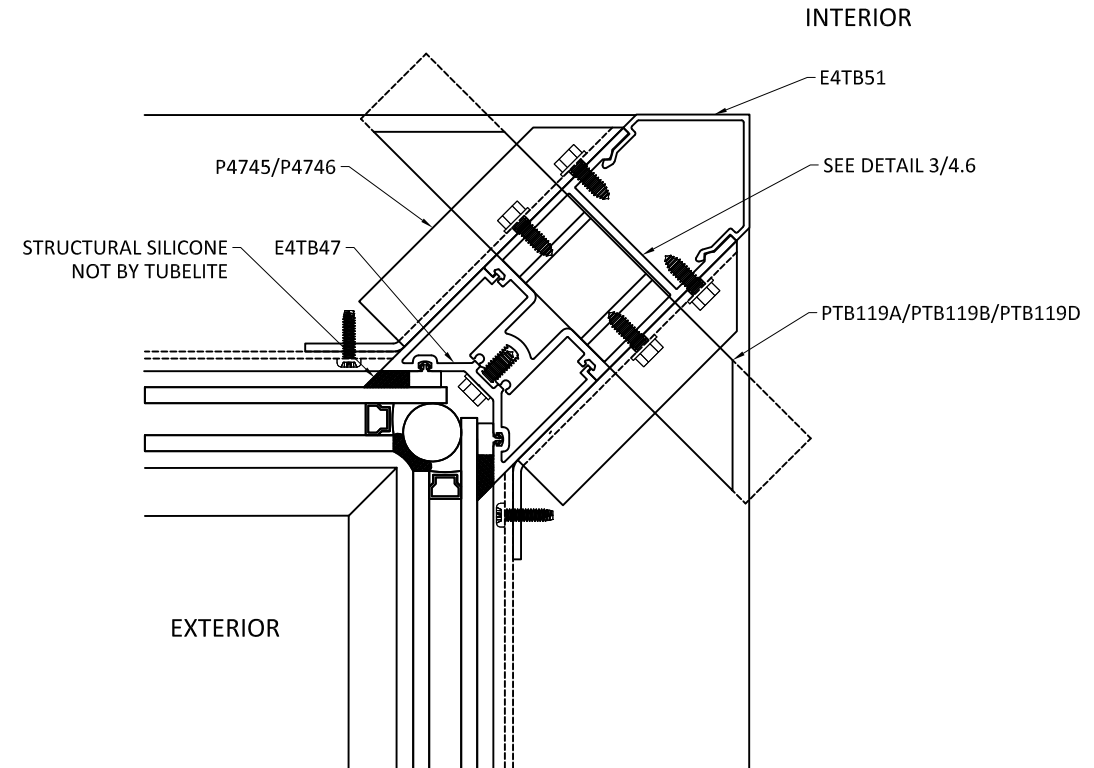
2 4.6 INSIDE CORNER STRUCTURAL SILICONE GLAZE
