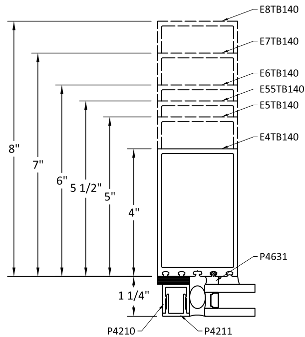
JAMB STRUCTURAL SILICONE GLAZE
