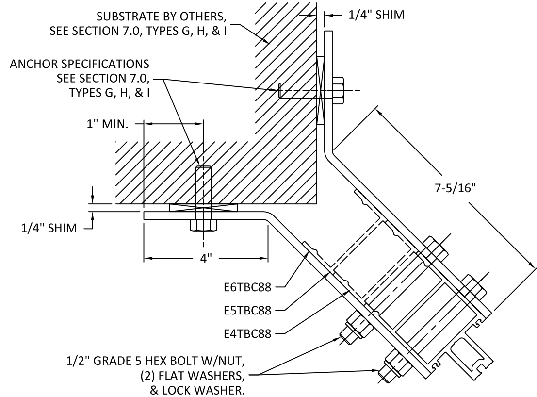
1 8.1 VERTICAL SECTION WIND/DEAD LOAD ANCHOR AT CORNER
